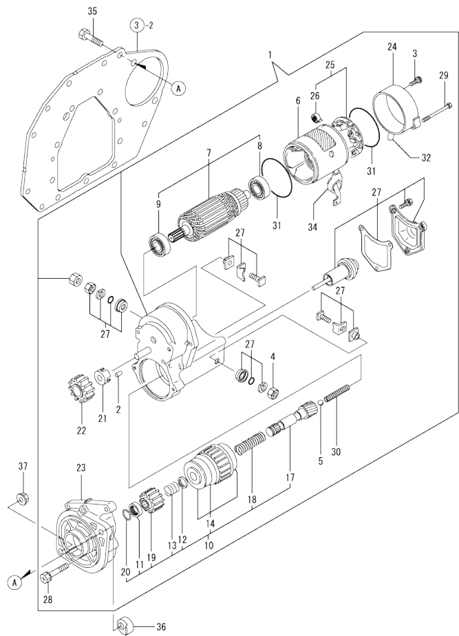
Fig.14. STARTING MOTOR
