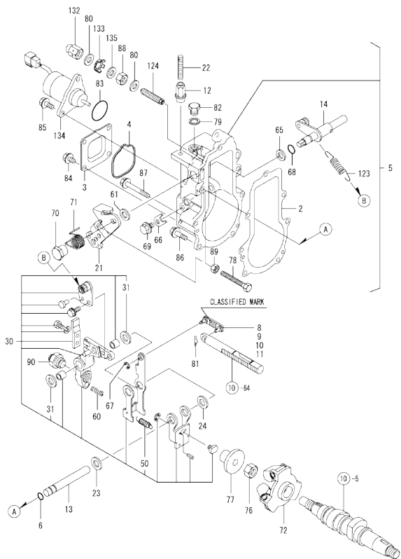
Fig.11. GOVERNOR
