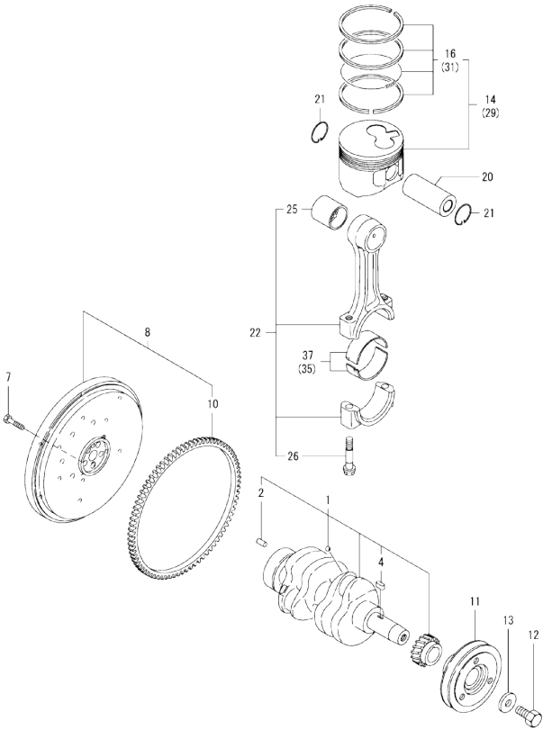
Fig.7. CRANKSHAFT & PISTON
