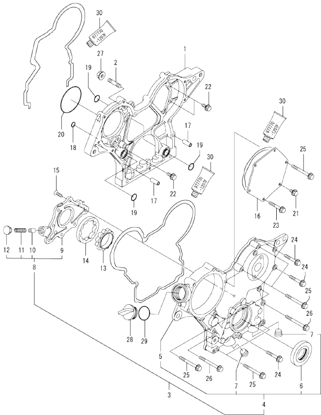
Fig.2. GEAR HOUSING
