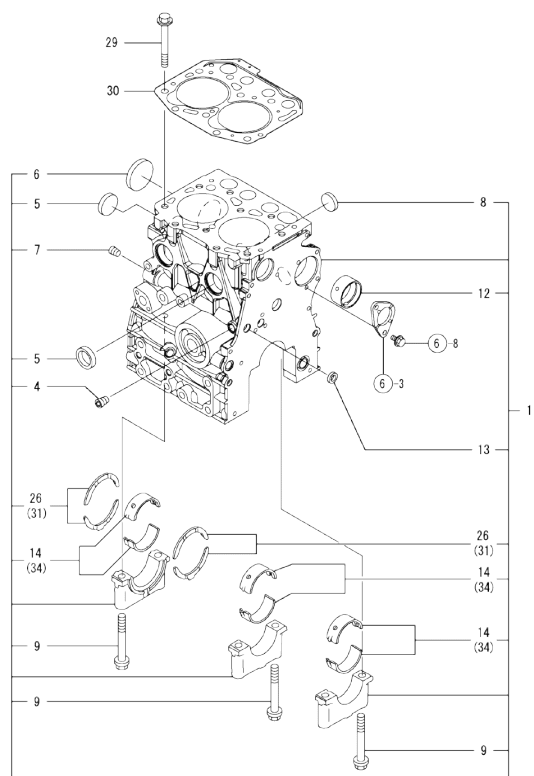
Fig.1. CYLINDER BLOCK
